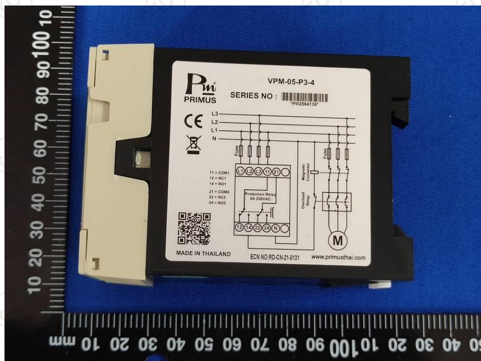
Photo 2- External view
