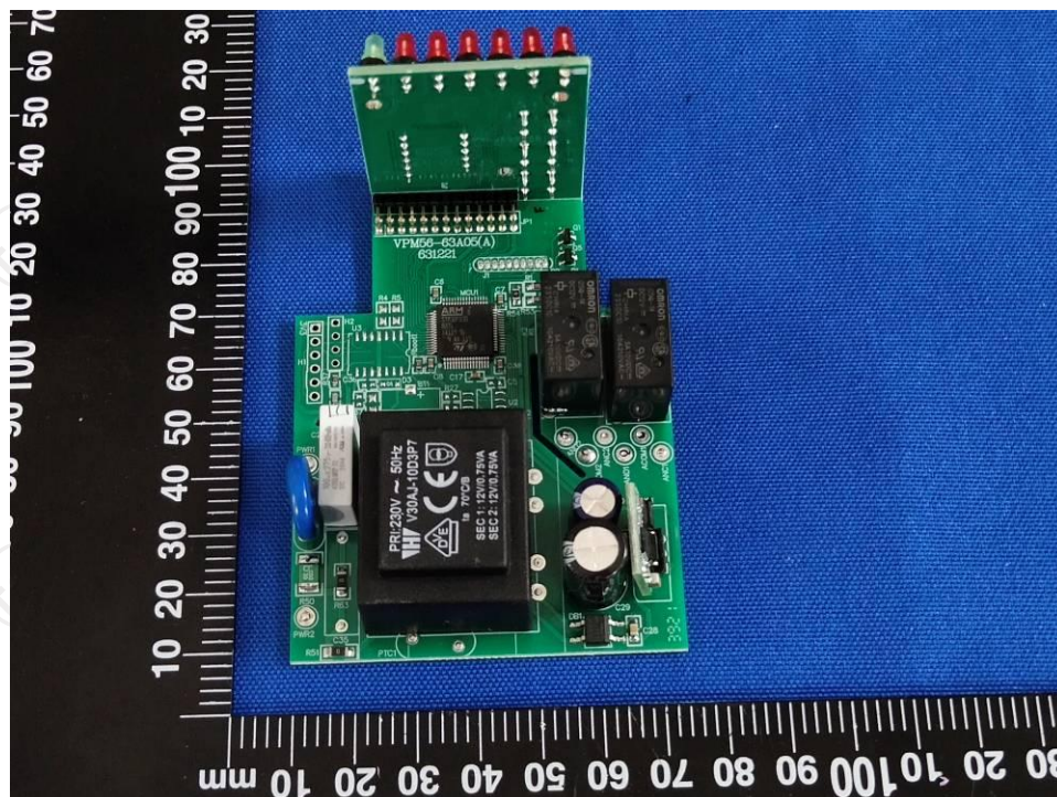
Photo 13- Internal view
