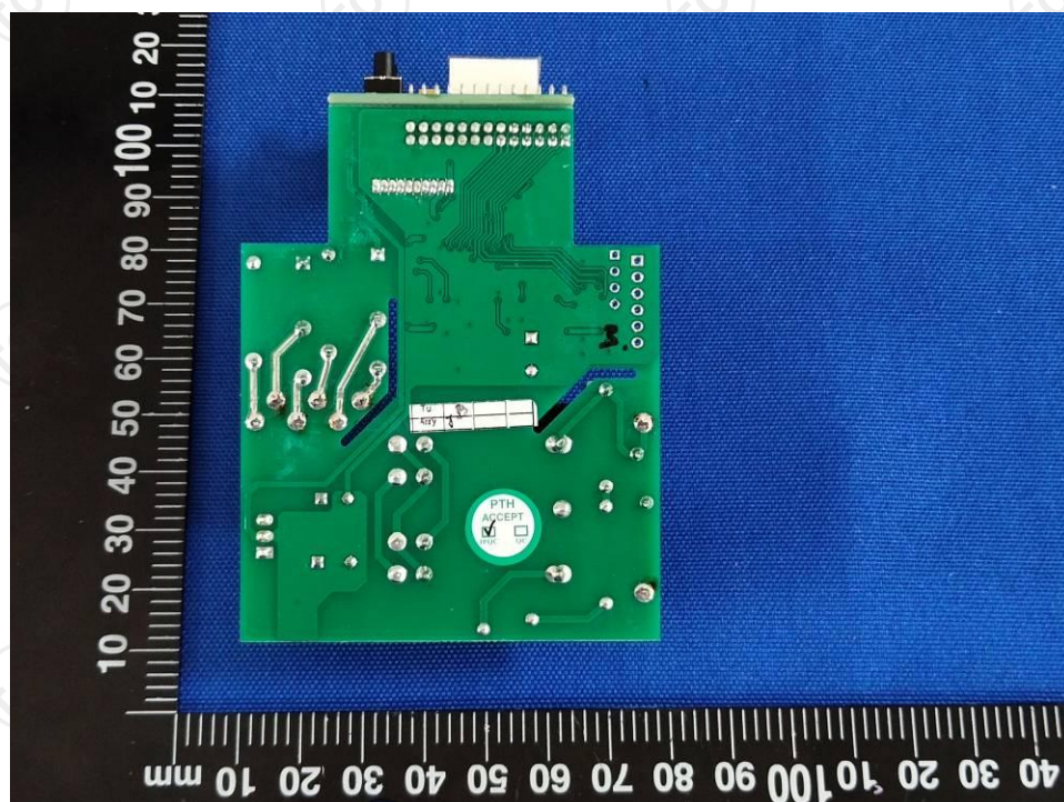
Photo 14- Internal view
