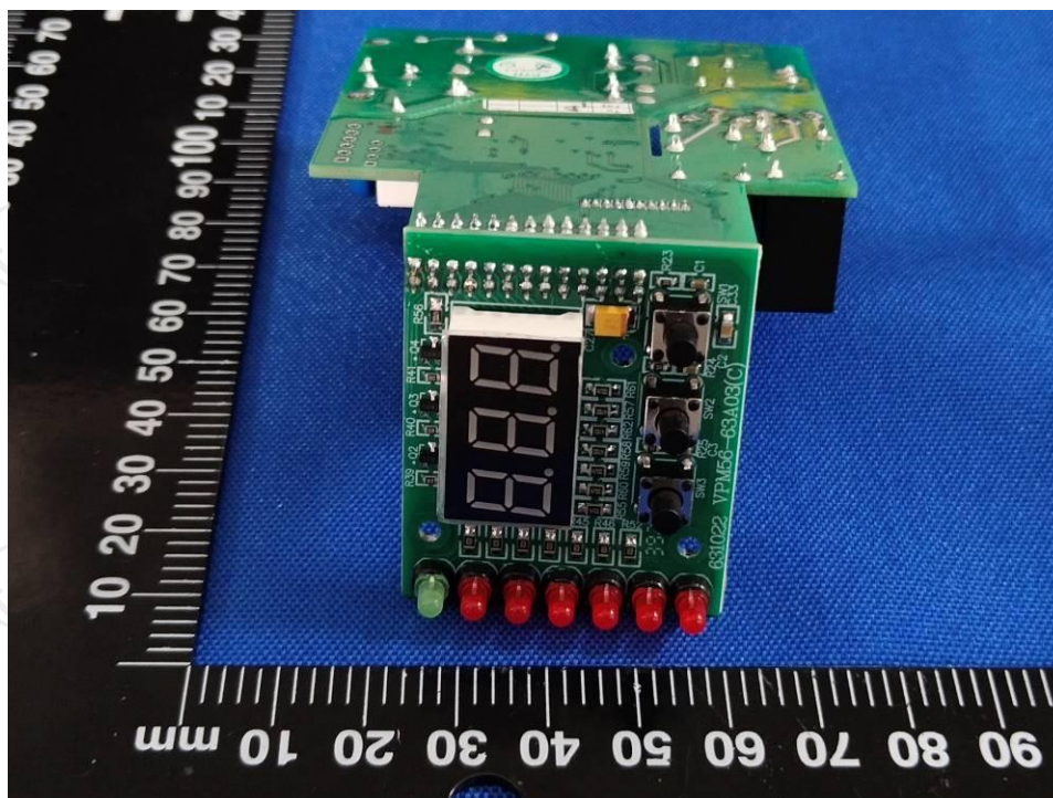
Photo 15- Internal view
