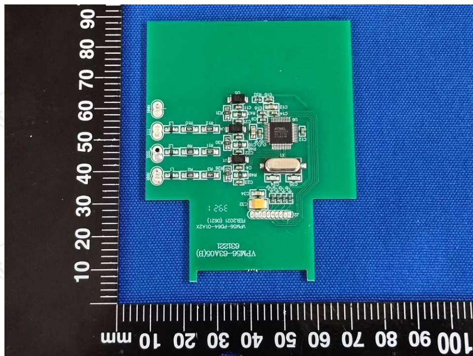
Photo 11- Internal view
