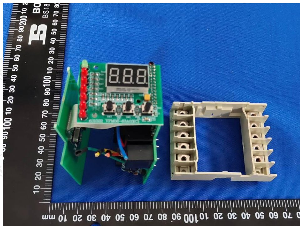
Photo 9- Internal view
