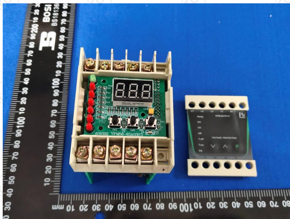
Photo 8- Internal view
