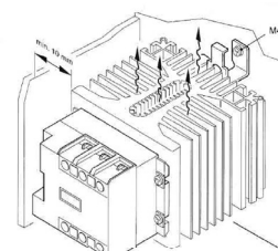
Mounting a contactor
