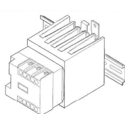
Mounting a contactor on a DIN rail EN50022 (omega)
