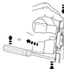
Removing a contactor by hand or with a screwdriver
