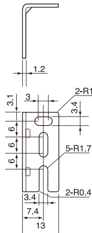
Tiny reflector P45A
