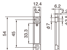
Tiny reflector P45A
