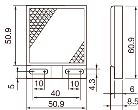
Standard reflector V-61
