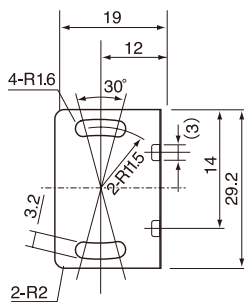
Standard reflector V-61
