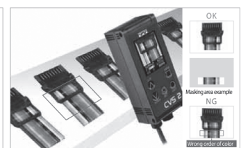
Checking order of the color of wires
